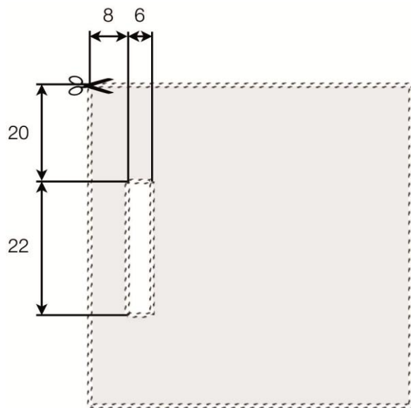
Hole template for the panel [mm]
